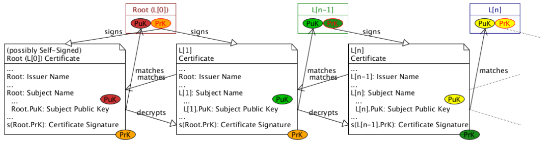
Figure 4.3: A Certificate Chain
